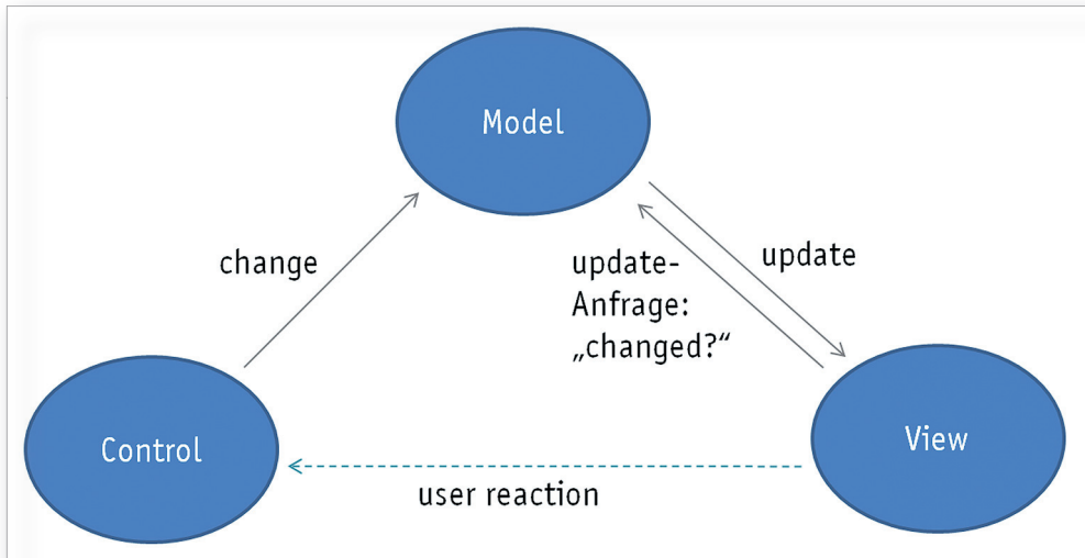
2 Model-View-Control Designpattern.
