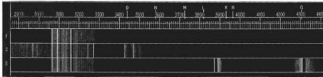
[Fig. 1] Line spectrum of hydrogen (Source: Huggins 1880, 577).
