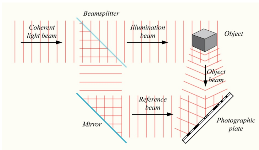
Fig. 1: Holography recording. https://upload.wikimedia.org/wikipedia/commons/7/77/Holograph-record.svg DrBob at the English-language Wikipedia, CC BY-SA 3.0 < http://creativecommons.org/licenses/by-sa/3.0/ >, via Wikimedia Commons.
